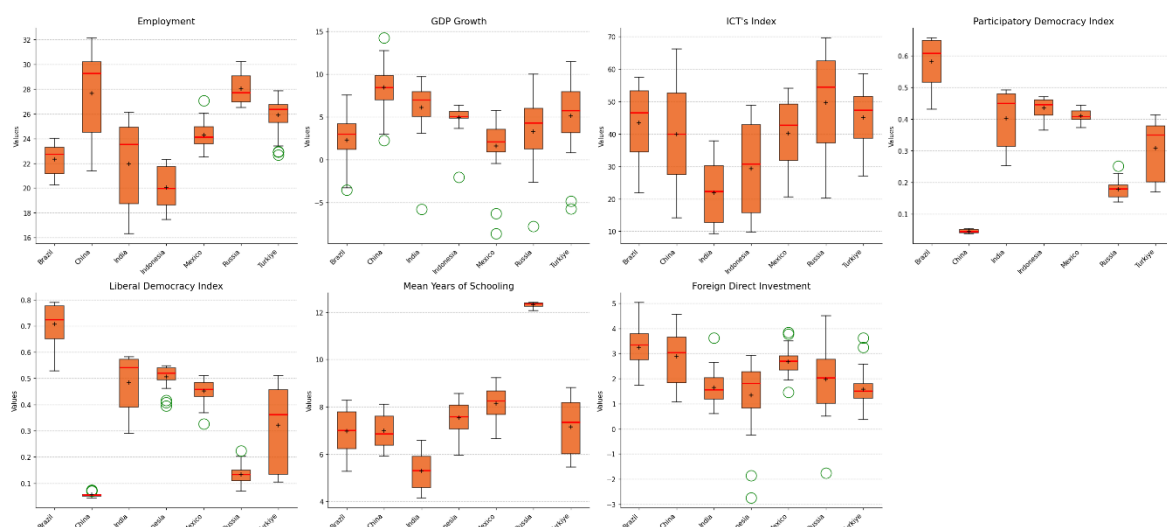
Figure 4 - Box plots of indicators for E7 Countries
