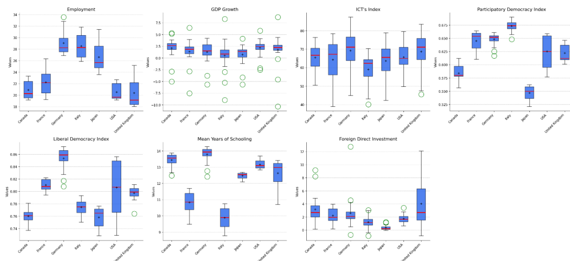
Figure 5 - Box plots of indicators for G7 Countries
