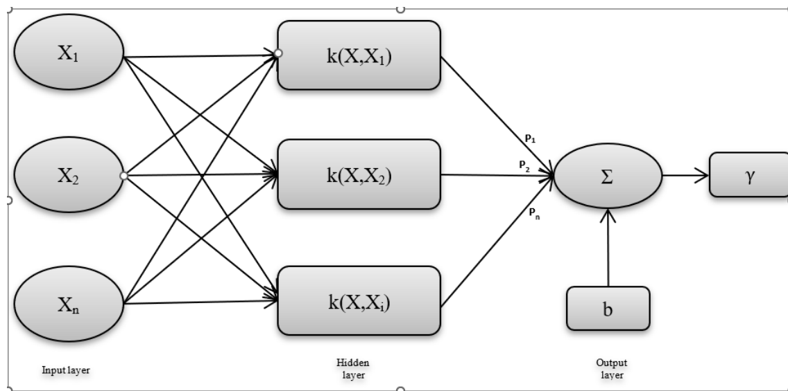
Figure 3 - Network operation of the SVM
