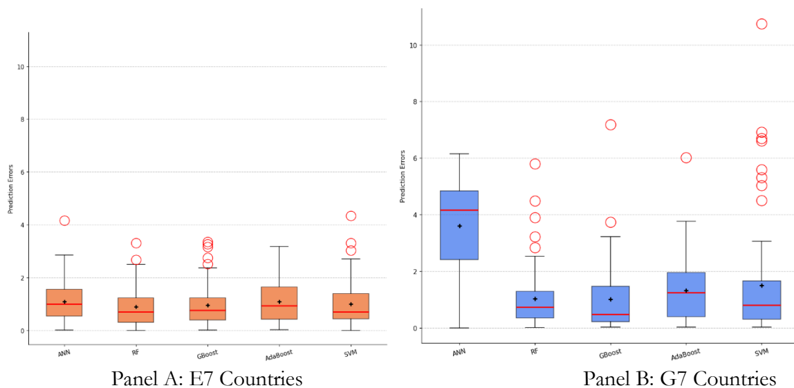
Figure 7 - Prediction Errors for E7 and G7 countries
