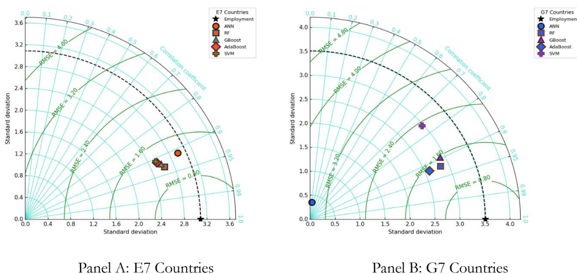
Figure 8 - Taylor diagrams for E7 and G7 countries
