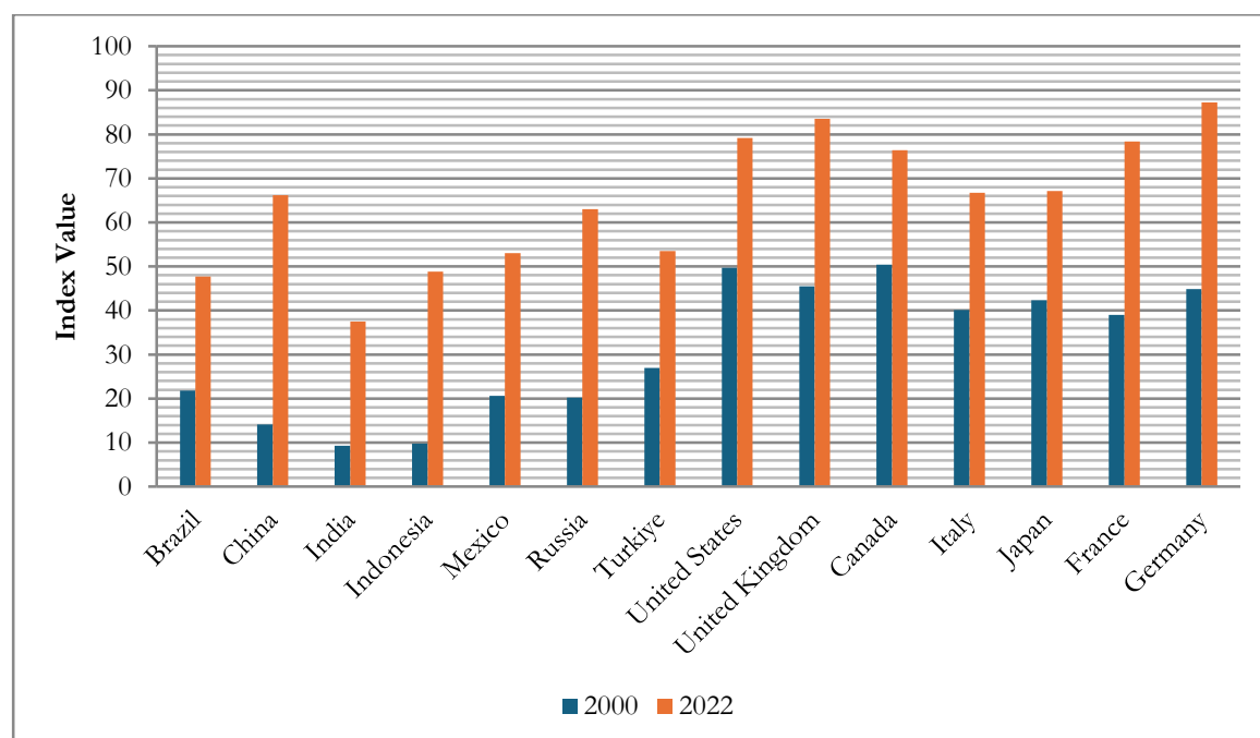
Figure 1 - ICTs Index in E7 and G7 countries
