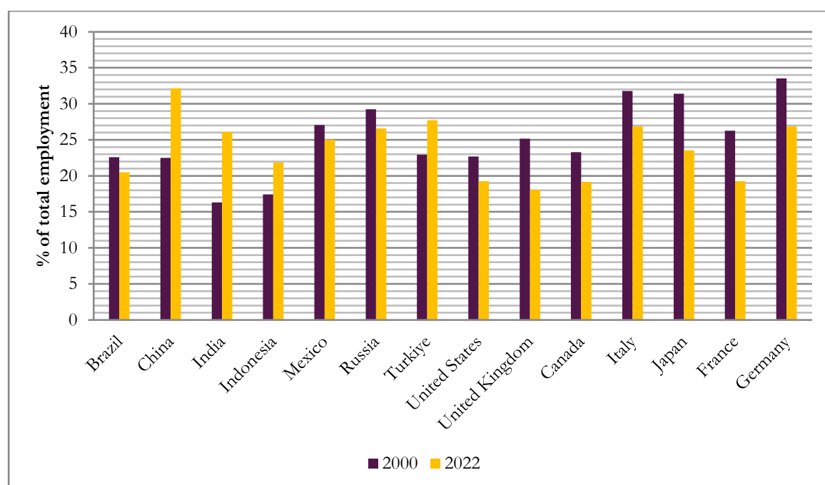
Figure 2 - Employment in industry in E7 and G7 countries
